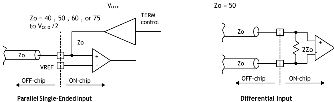
Figure 3.1. On-Chip Termination
