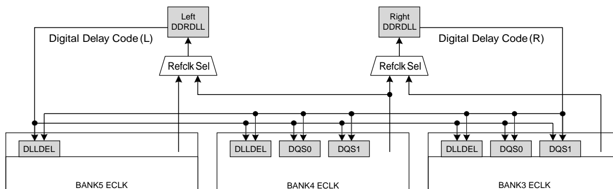
Figure 2.12. Certus-NX DDRDLL Architecture
