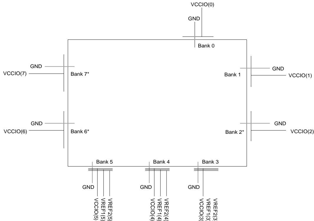
Figure 2.27. sysI/O Banking
