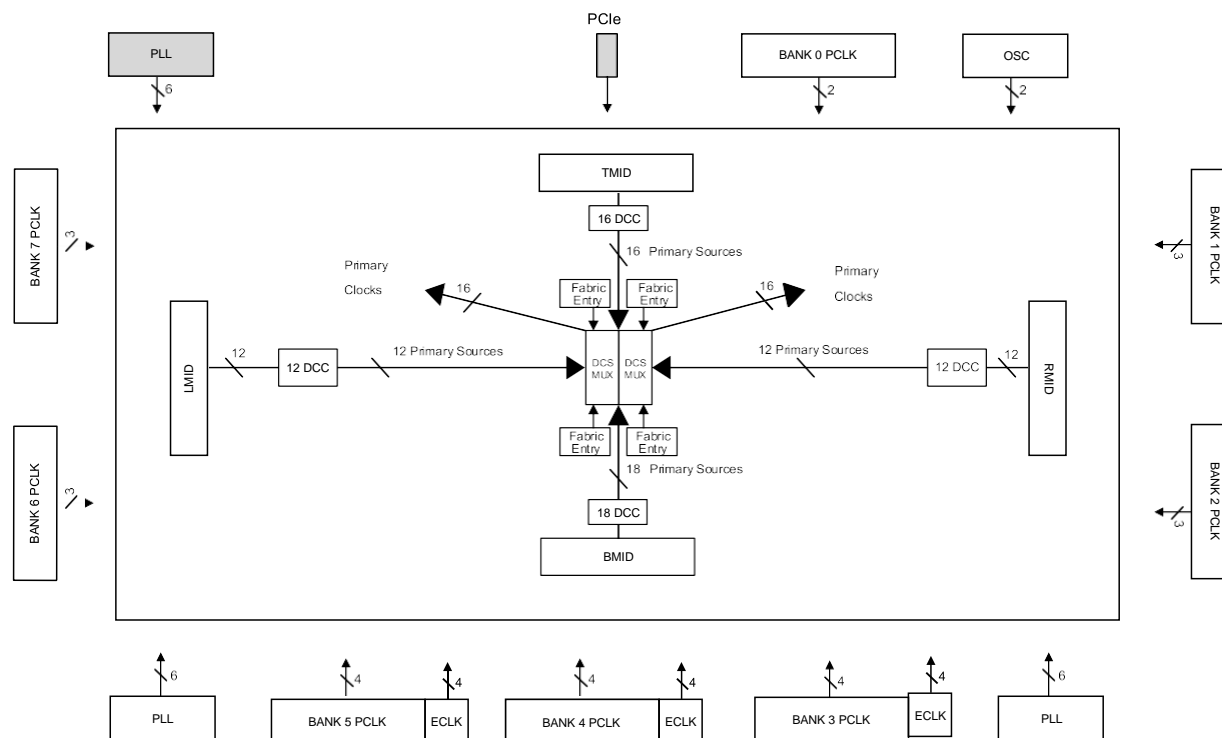
Figure 2.7. Clocking
