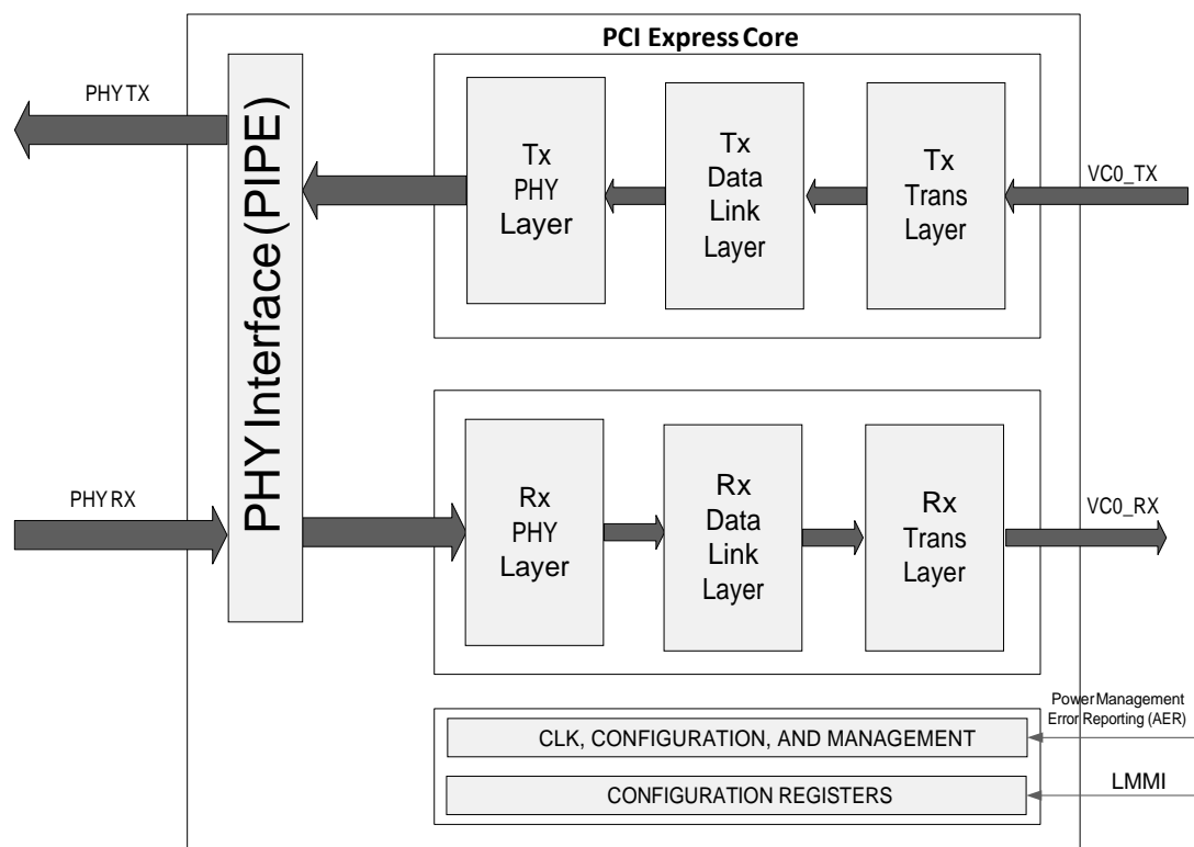
Figure 2.28. PCIe Core
