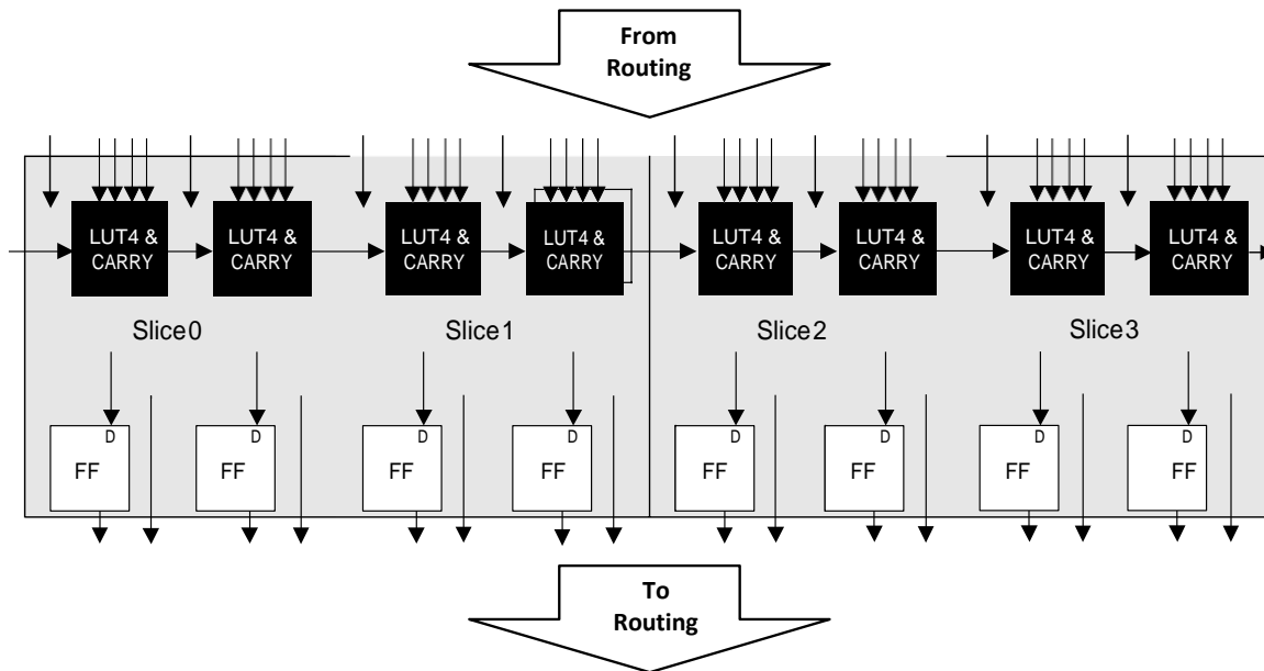
Figure 2.3. PFU Diagram
